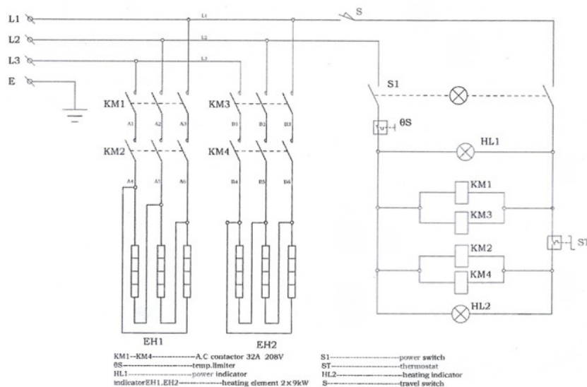
Electrical Diagram:
